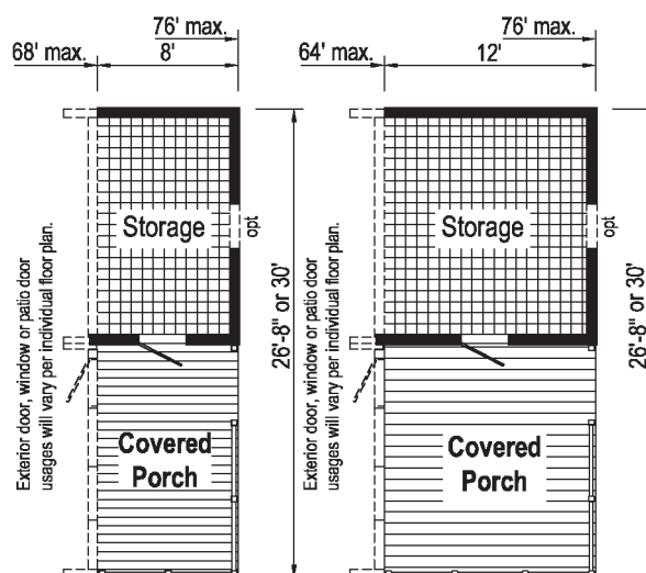
8' (YS) or 12' (XS) Covered Porch with Storage (Extended Floor Application)
