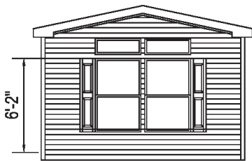
Double 3658 Windows with Transom
