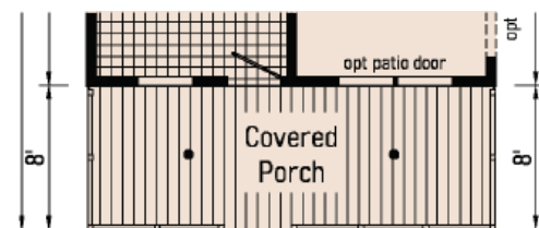
Optional 8' Covered Porch Model 3A2602-EY
