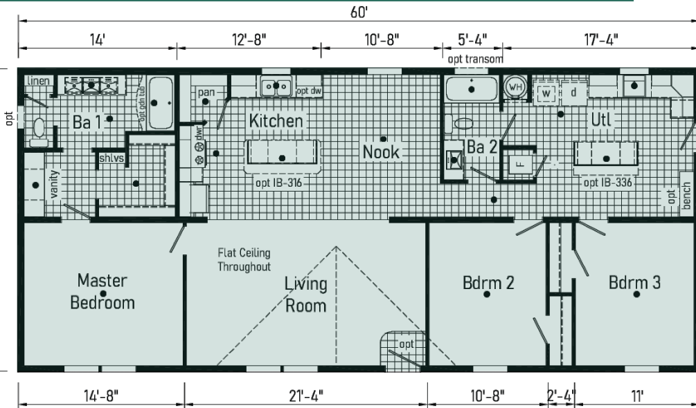
Curb Side Exterior Options
