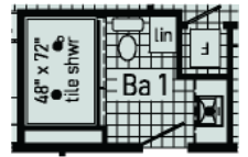
Optional 4'x6' Walk-In Tile Shower
