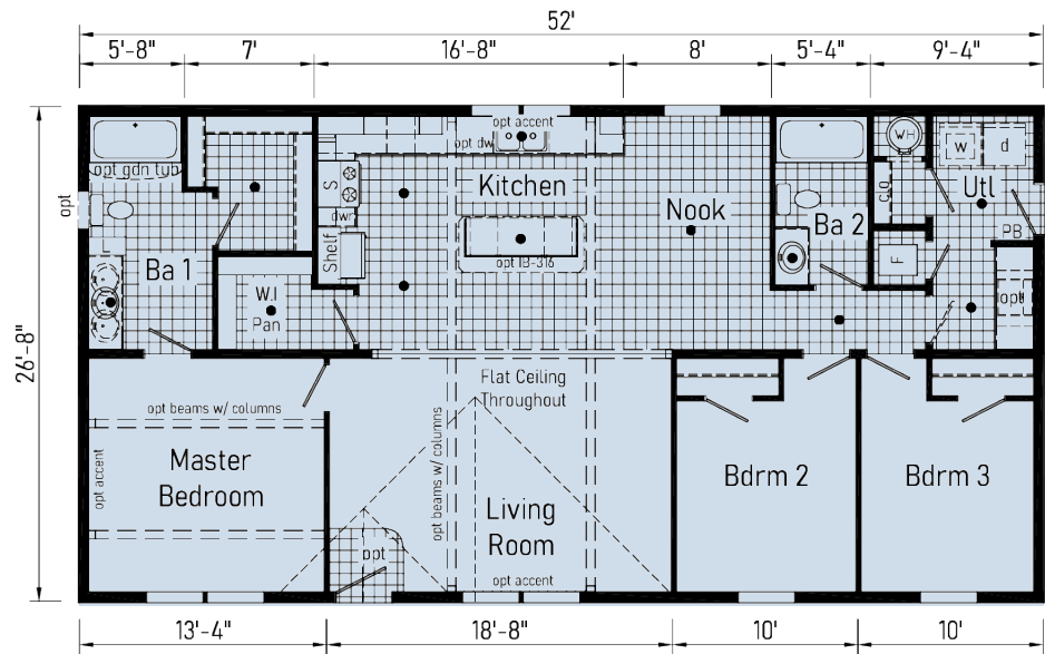
Optional Walk-Thru Pantry Cabinet
