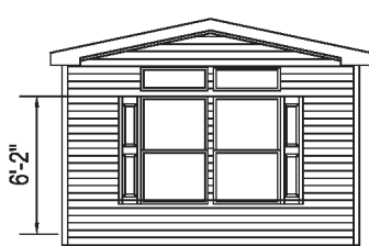
Double 3658 Windows with Transom
